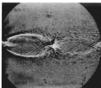
B. Shadowgraph of air into air
